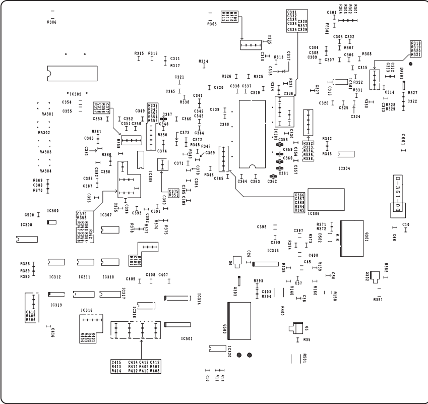
Solder Side
