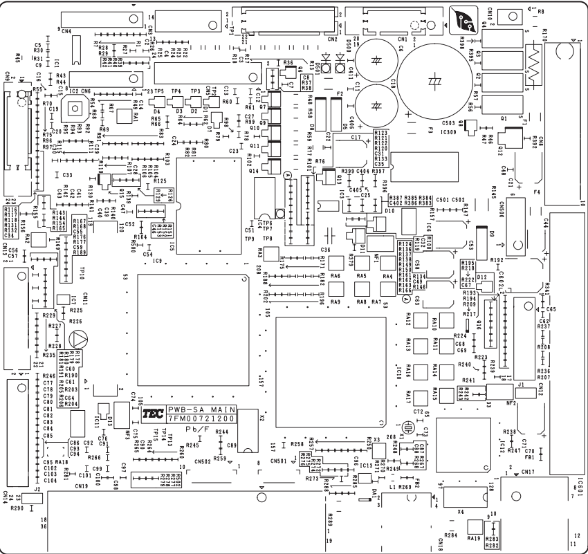
Parts Side
