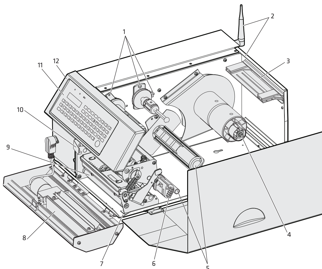
PX6i Spare Parts Overview
